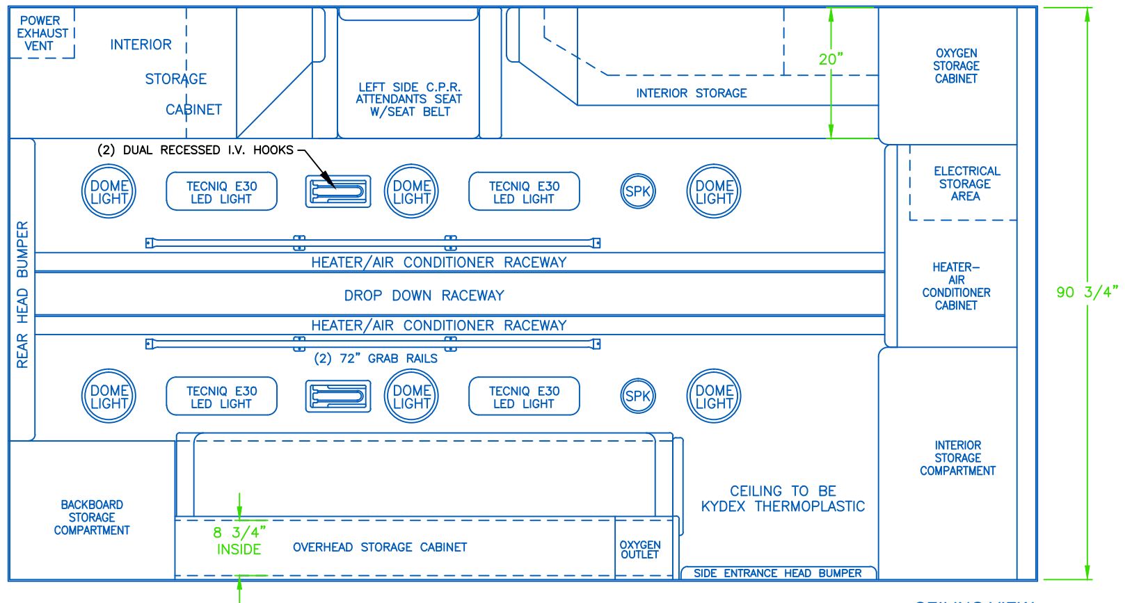
CEILING VIEW
