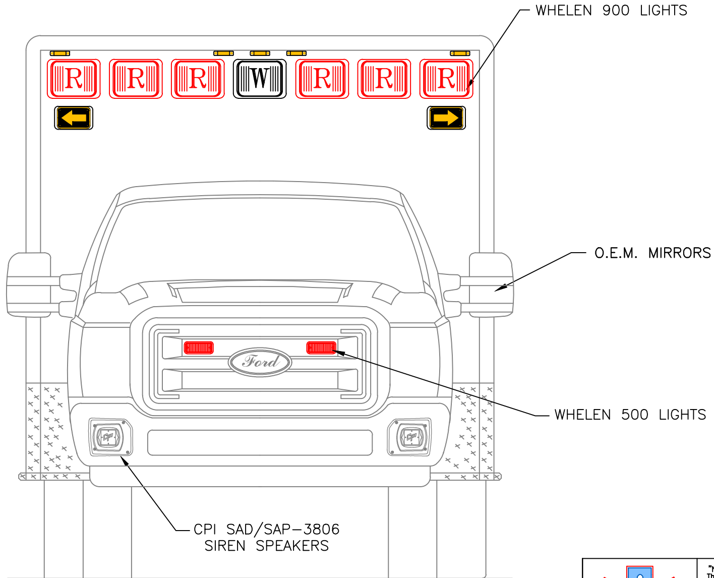
FRONT VIEW
