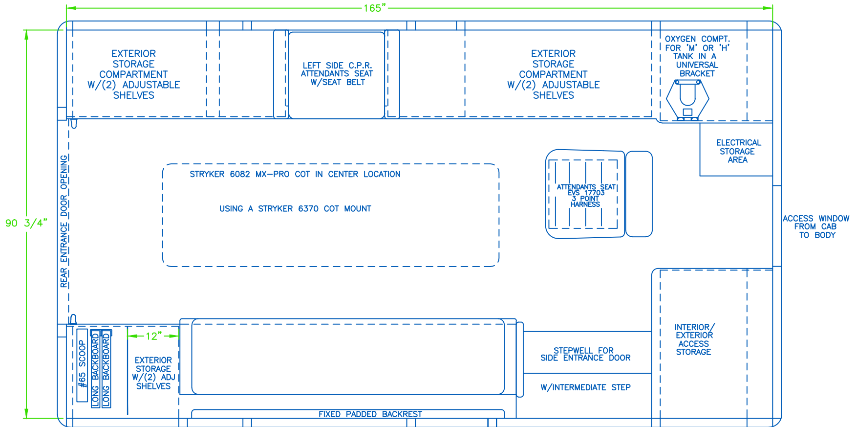
FLOOR PLAN
