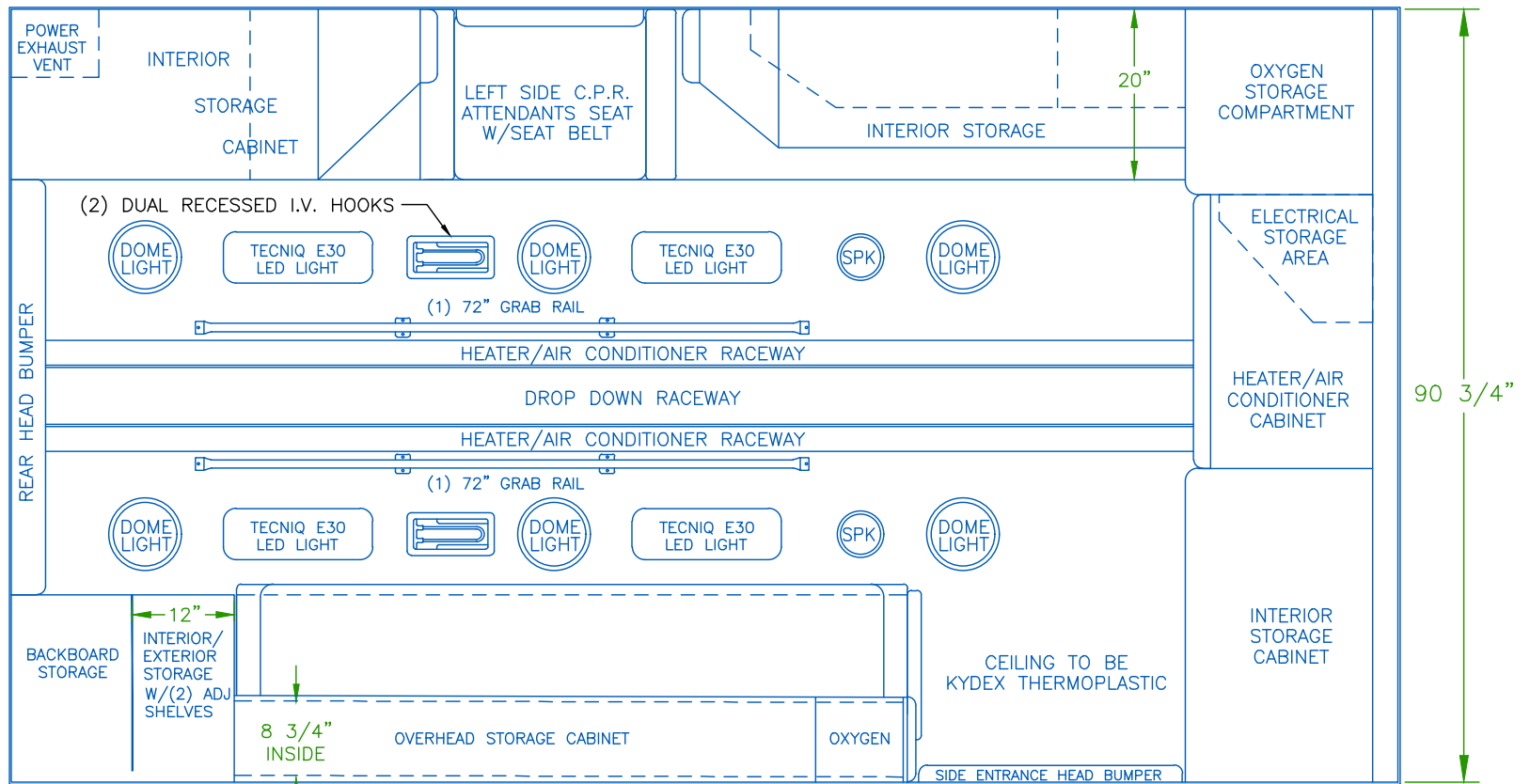
CEILING VIEW
