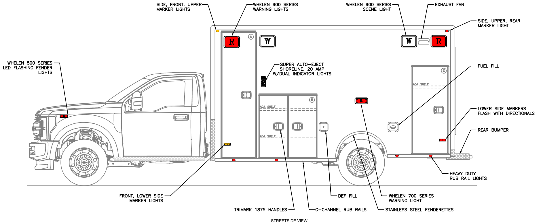
STREETSIDE VIEW
