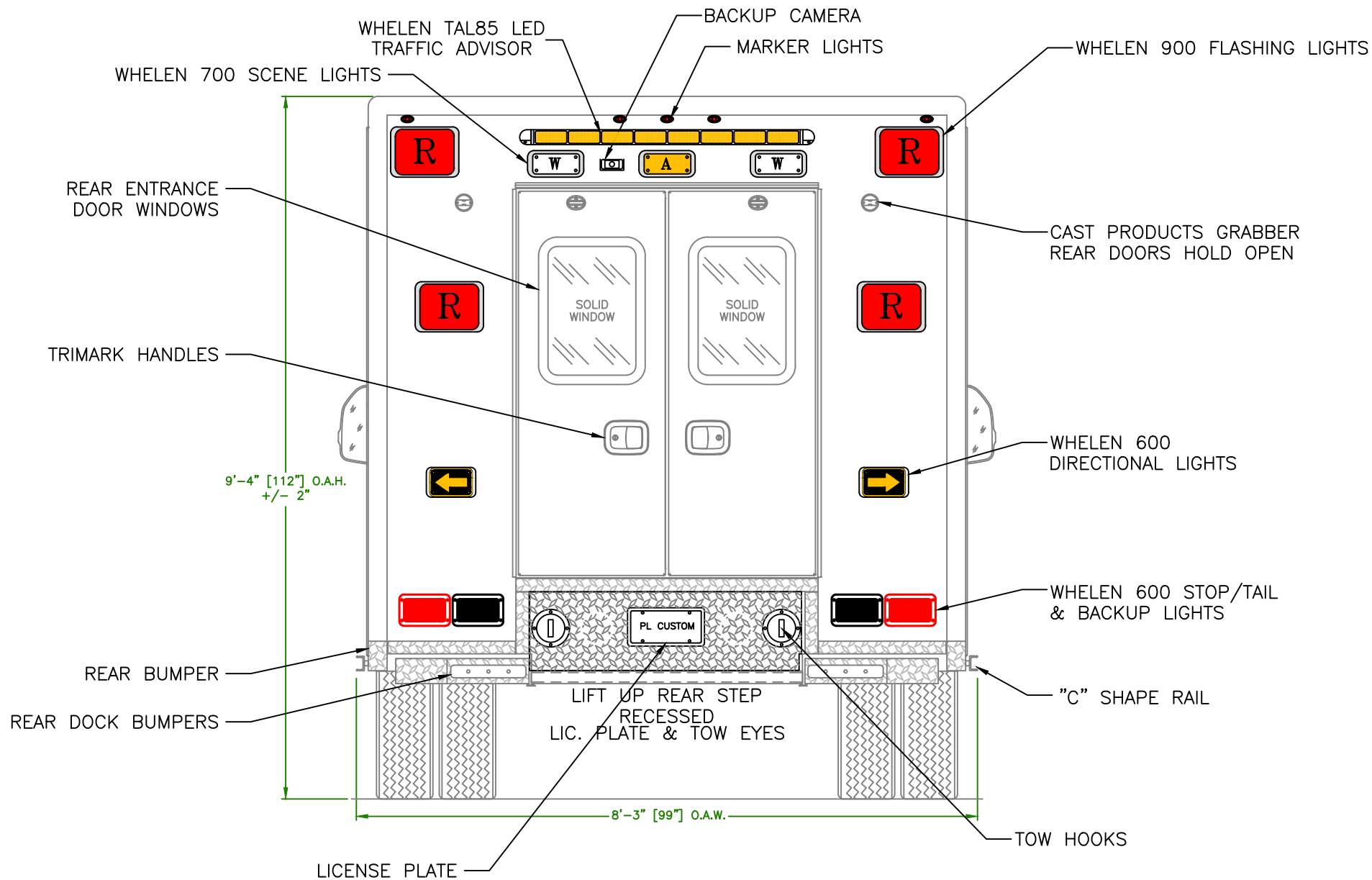
REAR VIEW
