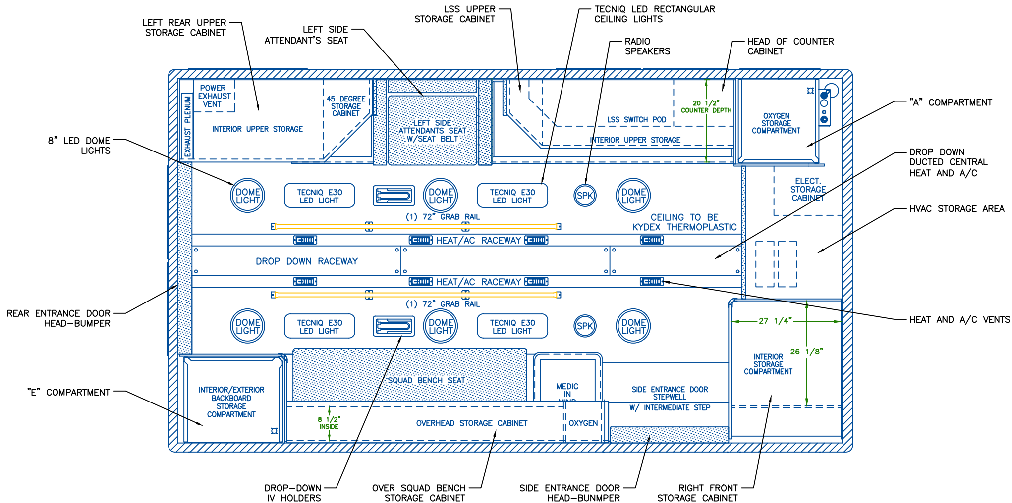
CEILING VIEW
